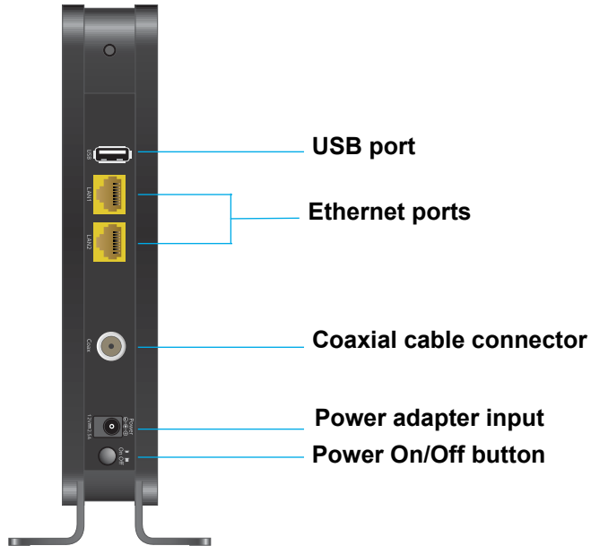
Figure 3. C3000v2 modem router rear panel
