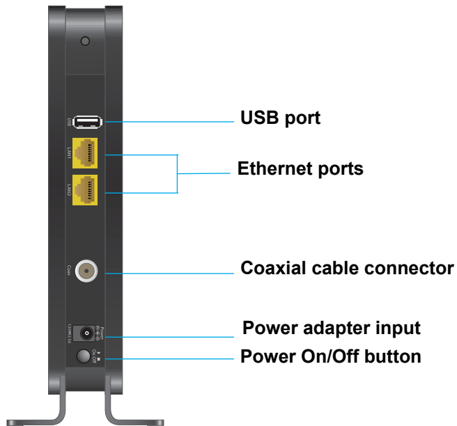
Figure 5. C3700v2 modem router rear panel
